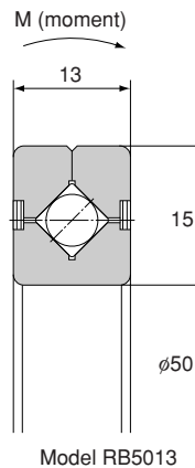
Cross-Roller Ring
