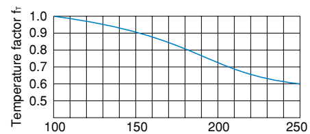
Fig. 1 Temperature Factor (f T )
