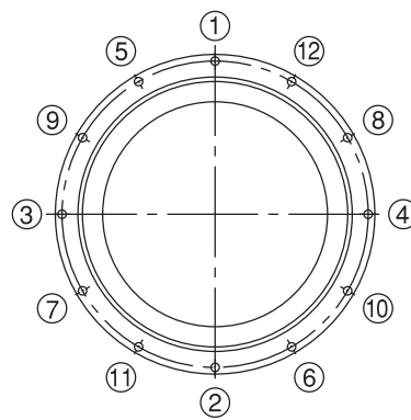
Fig. 1 Tightening Order
