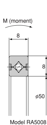
Model RA5008
