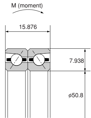
Angular ball bearing
