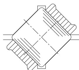
Symmetrical loaded areas Design with a spacer retainer
