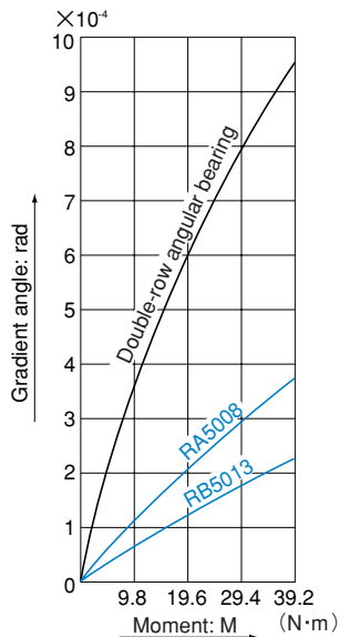
Moment Rigidity Diagram
